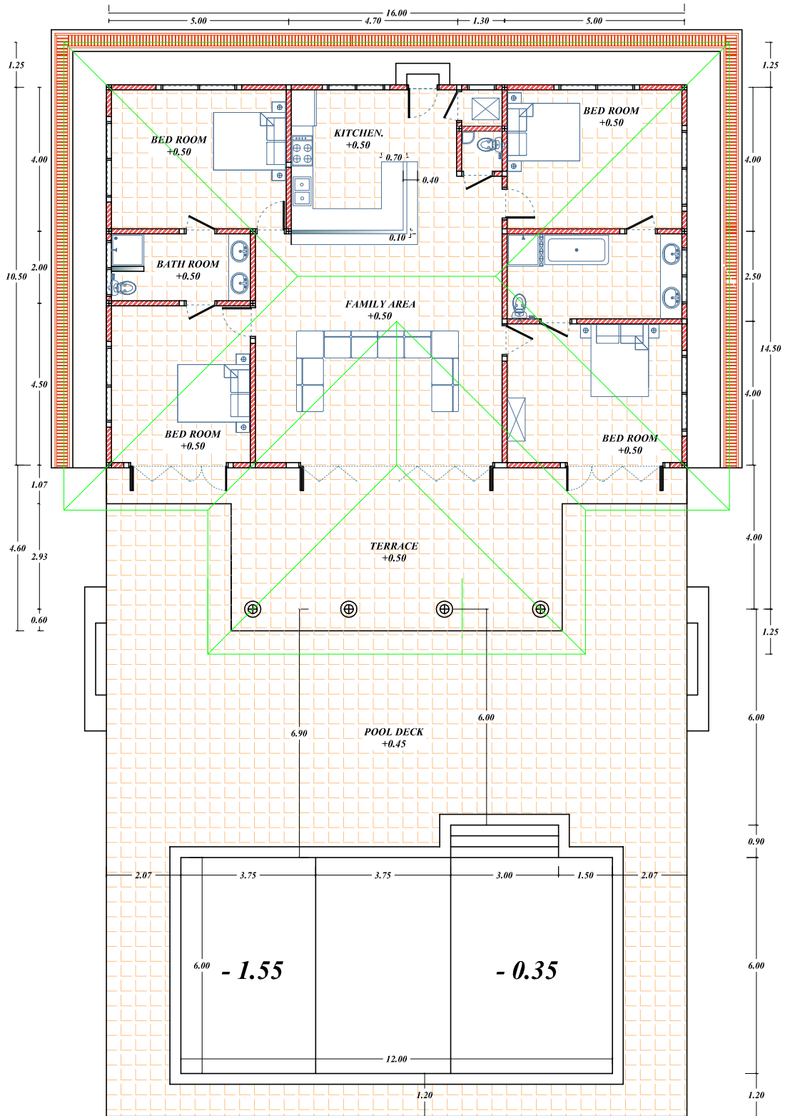
House Plan With Pool Scale 1 : 150
